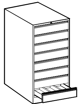
Type LS8/3/L-Spareinlagen 1350 h/654 b/450-650 t
